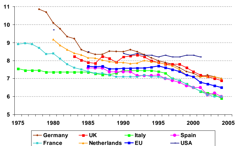
Figure 2.21: Specific consumption of new cars (litres/100km) 28 Consommation spécifique des automobiles neuves
